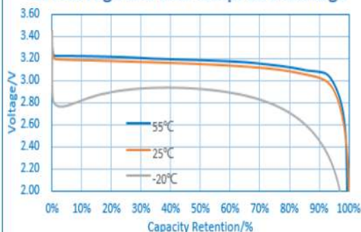
277Ah High and Low Temp. 1C Discharge
