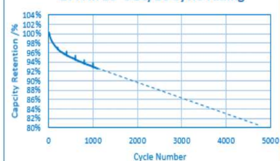
277Ah 25°C 1C/1C Cycle Fading
